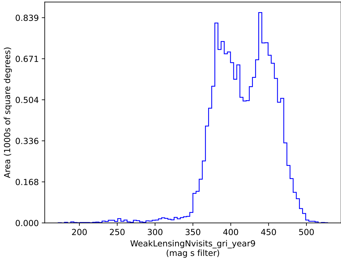
weather_cloudso16v3.4_10yrs gri band non-DD: WeakLensingNvisits_gri_year9
