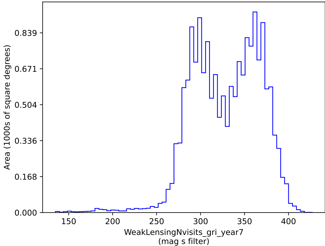
weather_cloudso16v3.4_10yrs gri band non-DD: WeakLensingNvisits_gri_year7
