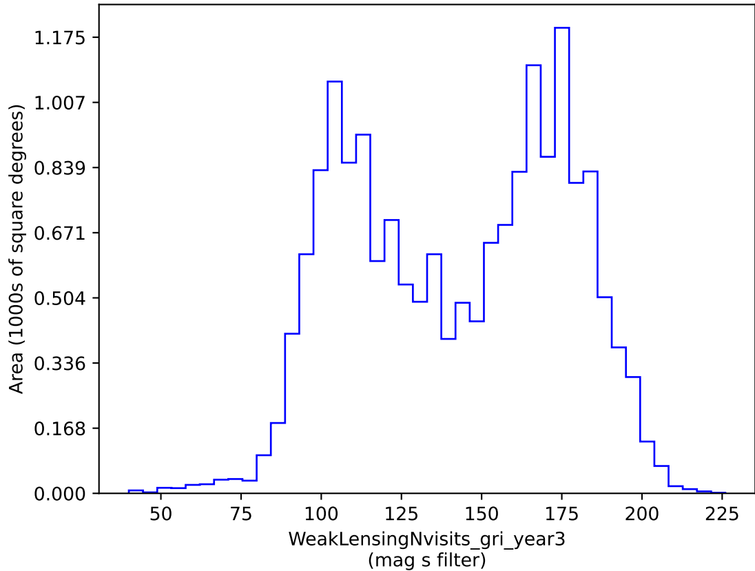
weather_cloudso16v3.4_10yrs gri band non-DD: WeakLensingNvisits_gri_year3
