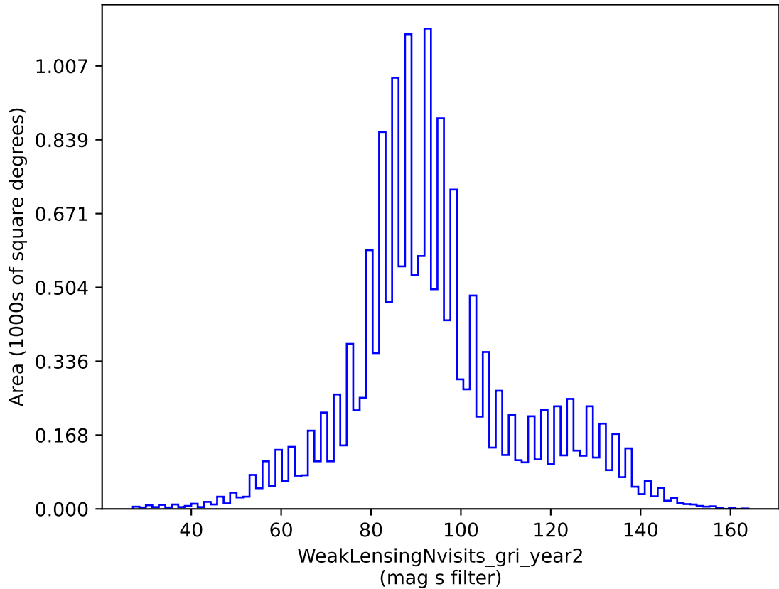
weather_cloudso16v3.4_10yrs gri band non-DD: WeakLensingNvisits_gri_year2
