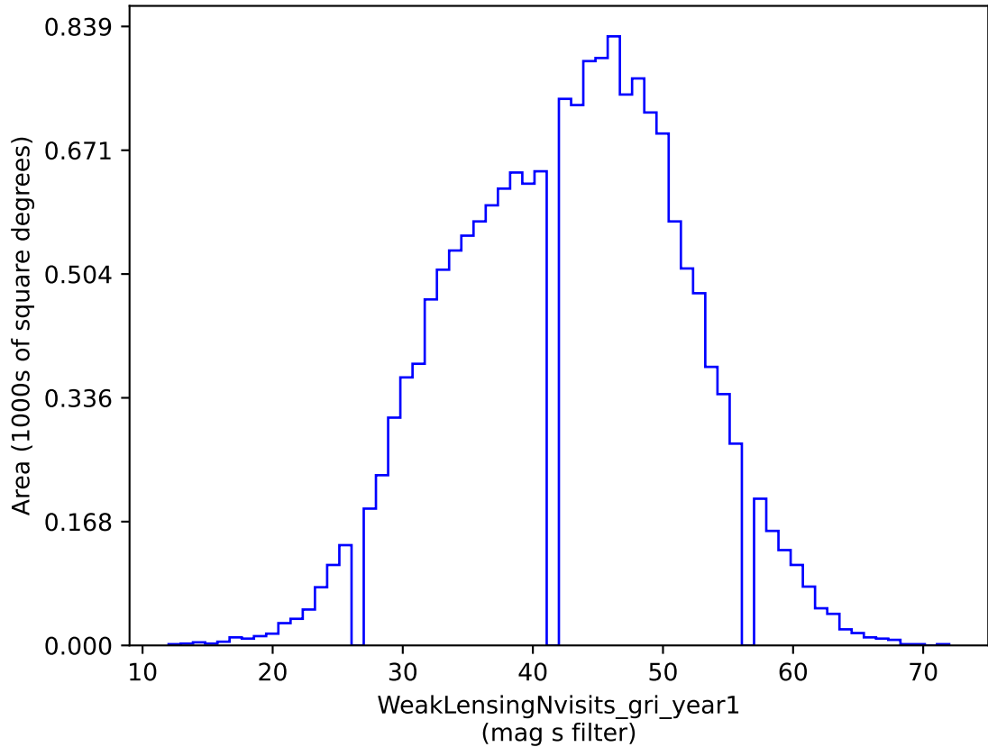
weather_cloudso16v3.4_10yrs gri band non-DD: WeakLensingNvisits_gri_year1
