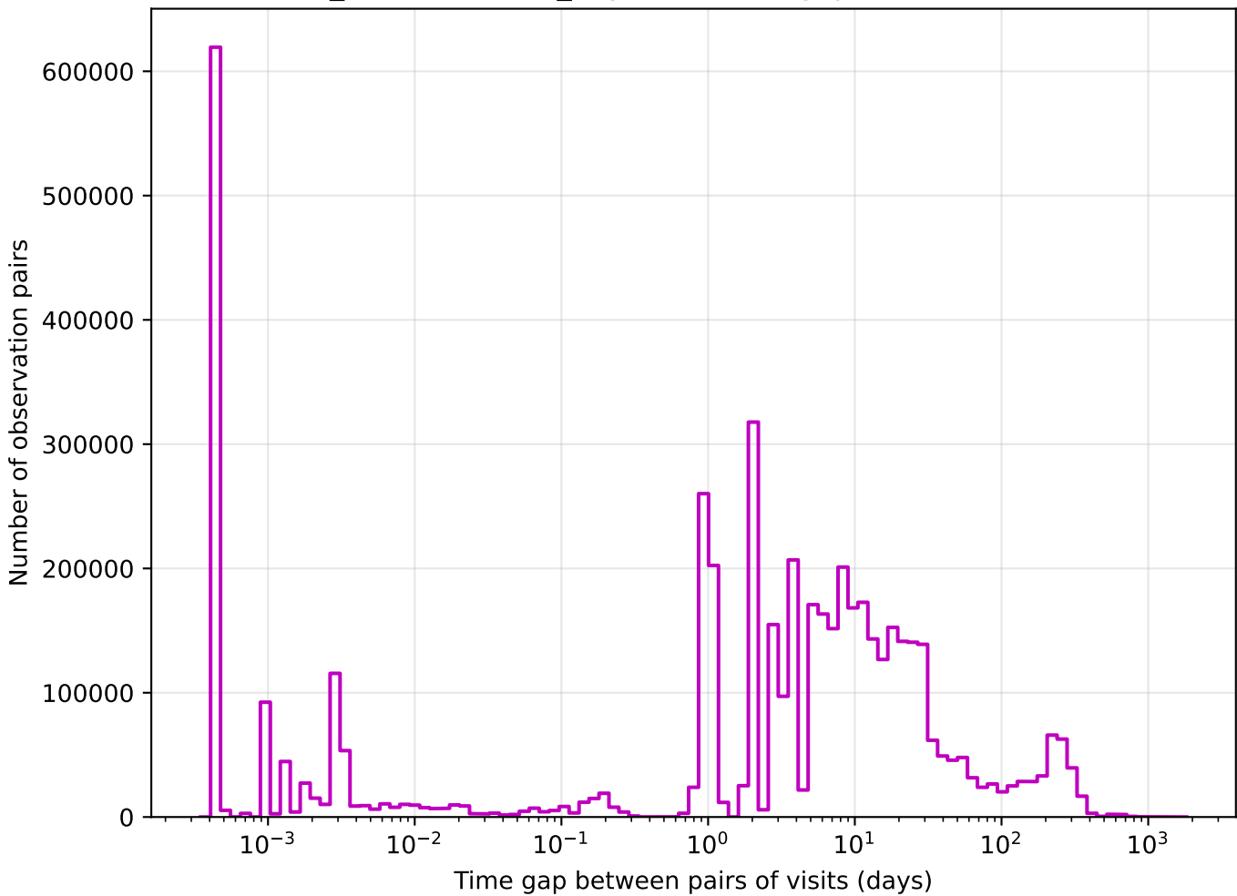
weather_cloudso16v3.4_10yrs z band: Tgaps observationStartMJD
