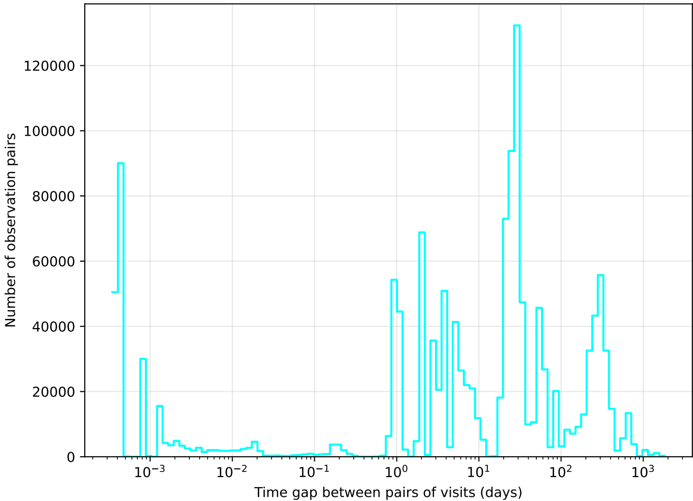
weather_cloudso16v3.4_10yrs u band: Tgaps observationStartMJD
