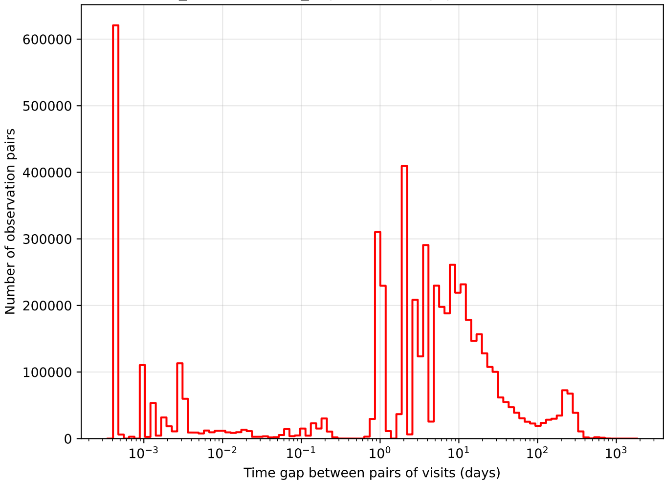
weather_cloudso16v3.4_10yrs i band: Tgaps observationStartMJD
