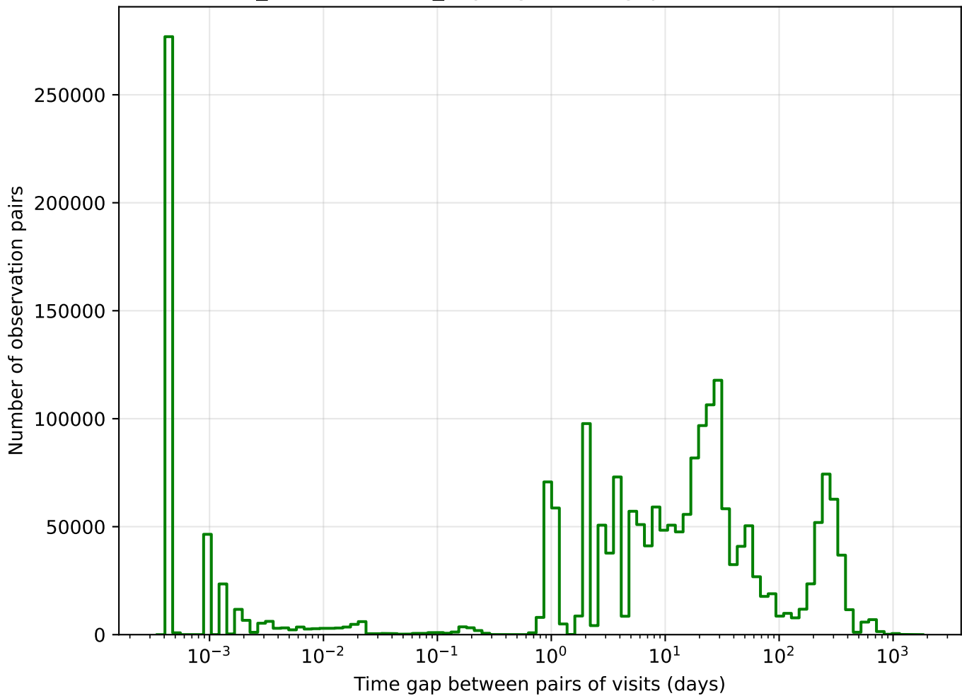
weather_cloudso16v3.4_10yrs g band: Tgaps observationStartMJD
