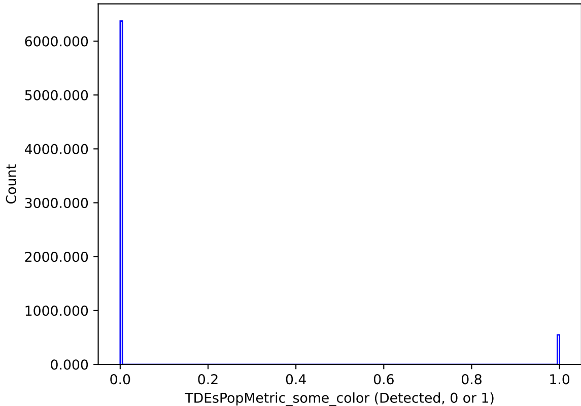
weather_cloudso16v3.4_10yrs : TDEsPopMetric_some_color
