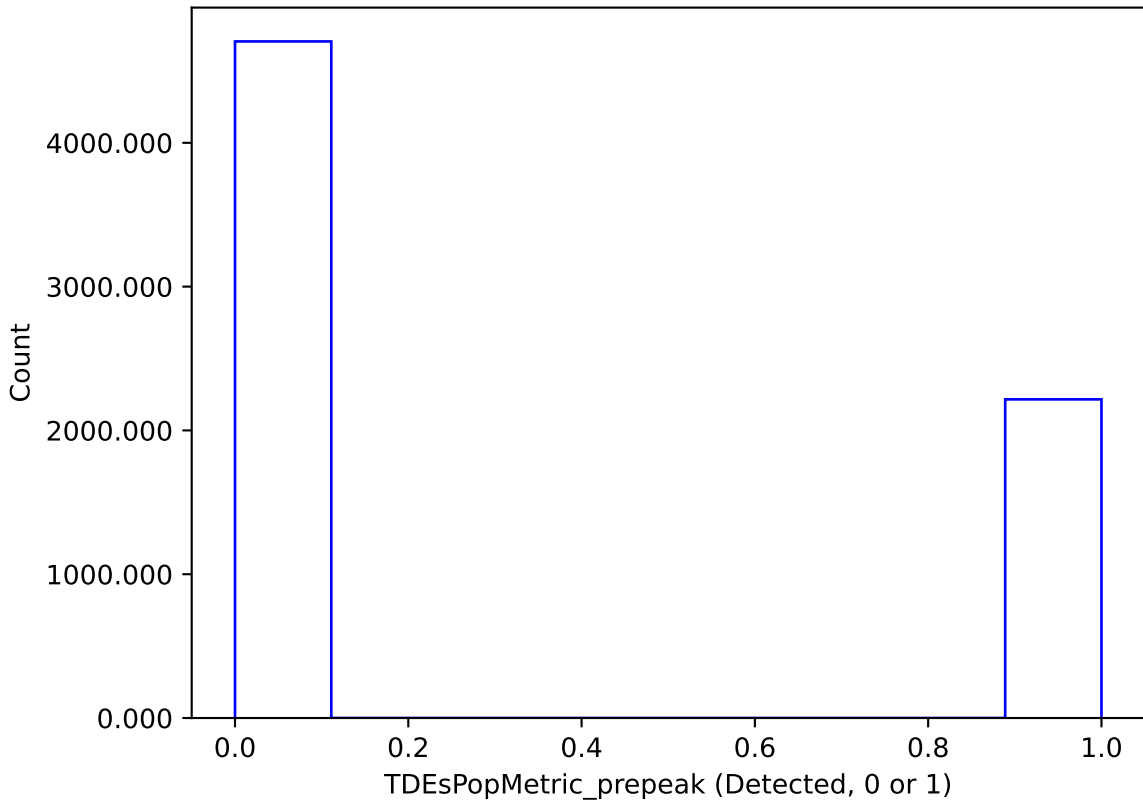
weather_cloudso16v3.4_10yrs : TDEsPopMetric_prepeak
