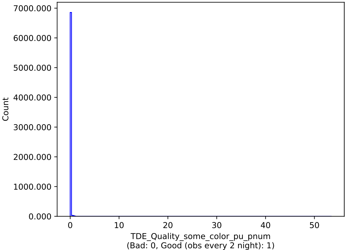
weather_cloudso16v3.4_10yrs : TDE_Quality_some_color_pu_pnum
