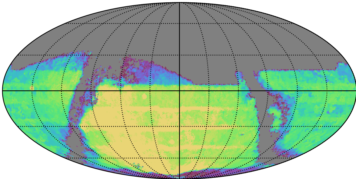
weather_cloudso16v3.4_10yrs : TDC_season
