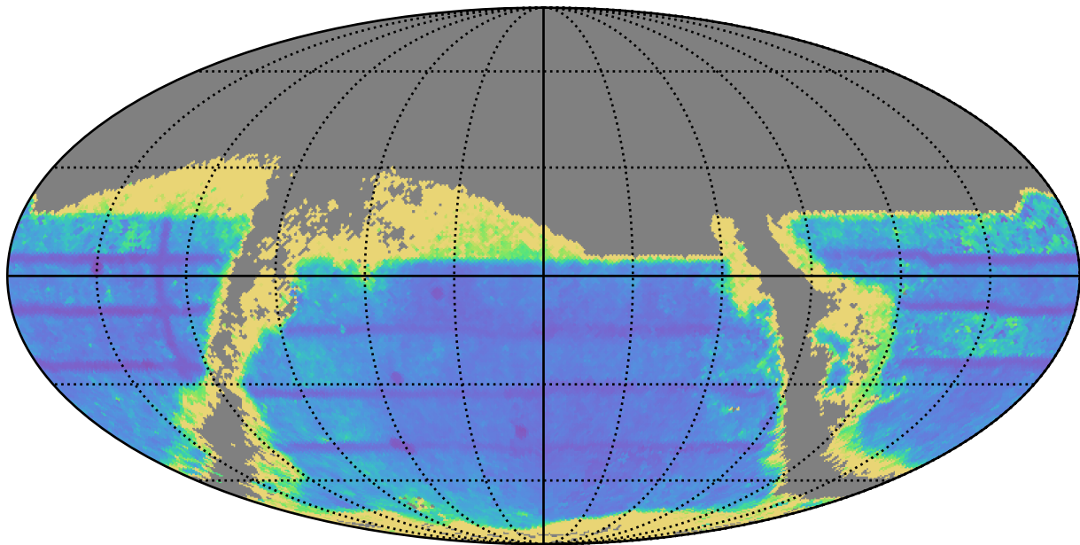
weather_cloudso16v3.4_10yrs : TDC_precision
