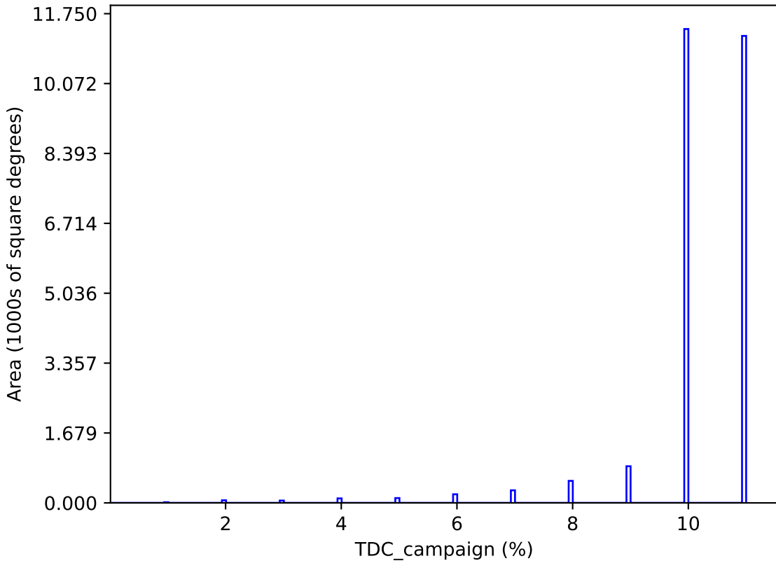
weather_cloudso16v3.4_10yrs : TDC_campaign
