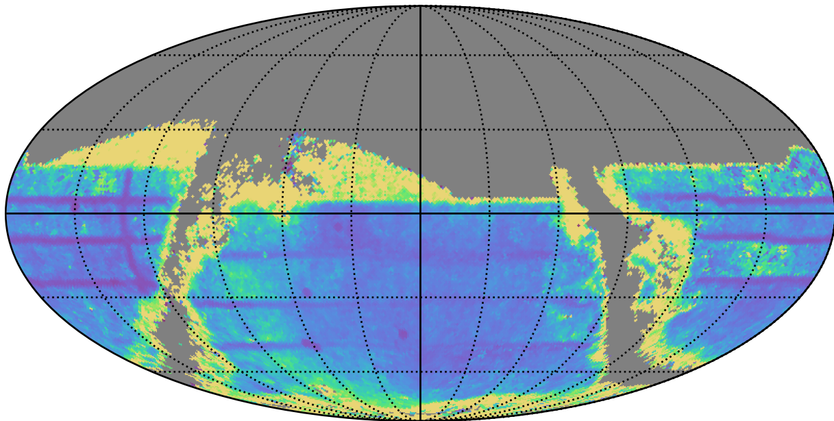
weather_cloudso16v3.4_10yrs : TDC_cadence
