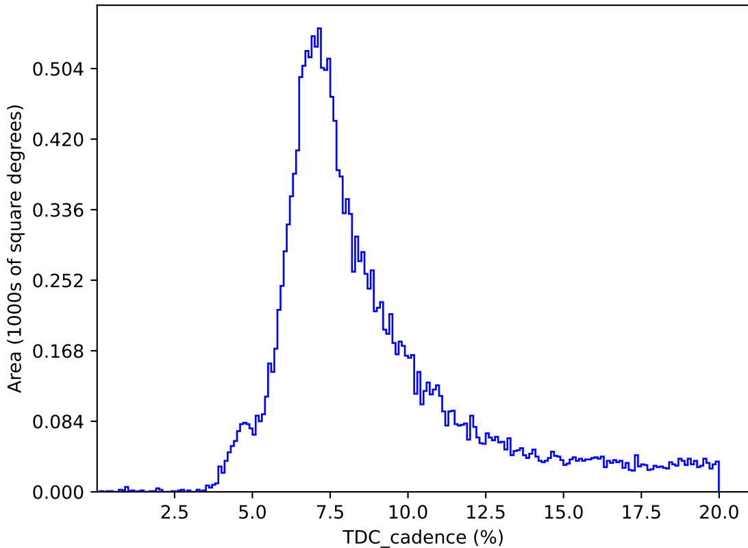
weather_cloudso16v3.4_10yrs : TDC_cadence
