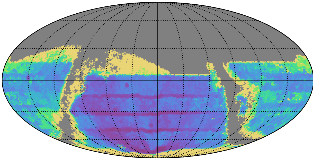
weather_cloudso16v3.4_10yrs : TDC_accuracy
