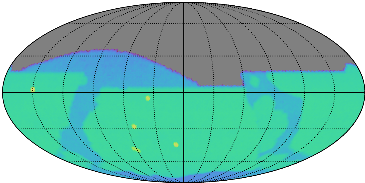
weather_cloudso16v3.4_10yrs z: SurfaceBrightLimit
