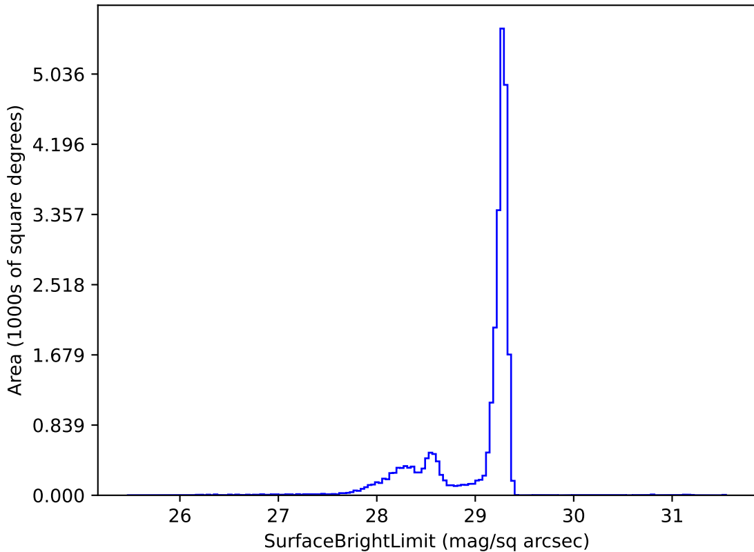
weather_cloudso16v3.4_10yrs z: SurfaceBrightLimit
