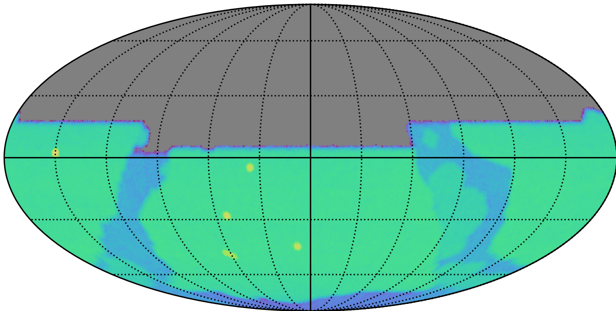
weather_cloudso16v3.4_10yrs y: SurfaceBrightLimit
