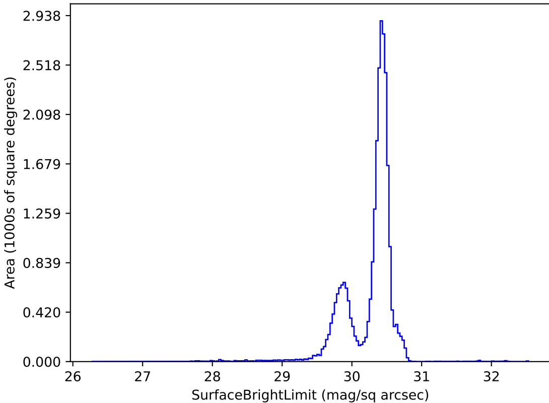
weather_cloudso16v3.4_10yrs g: SurfaceBrightLimit
