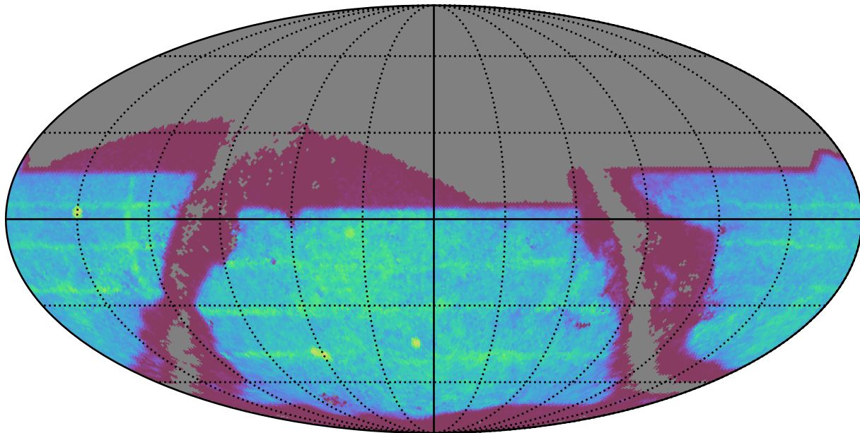
weather_cloudso16v3.4_10yrs : SNSLMetric
