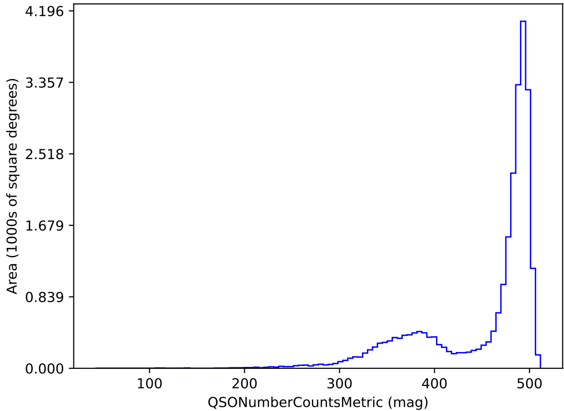
weather_cloudso16v3.4_10yrs z band and non-DD: QSONumberCountsMetric
