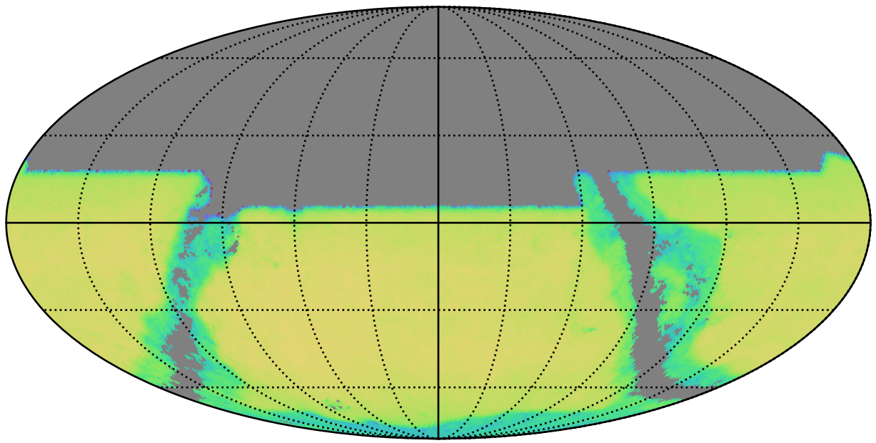
weather_cloudso16v3.4_10yrs y band and non-DD: QSONumberCountsMetric
