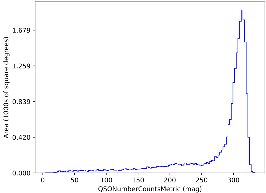
weather_cloudso16v3.4_10yrs u band and non-DD: QSONumberCountsMetric
