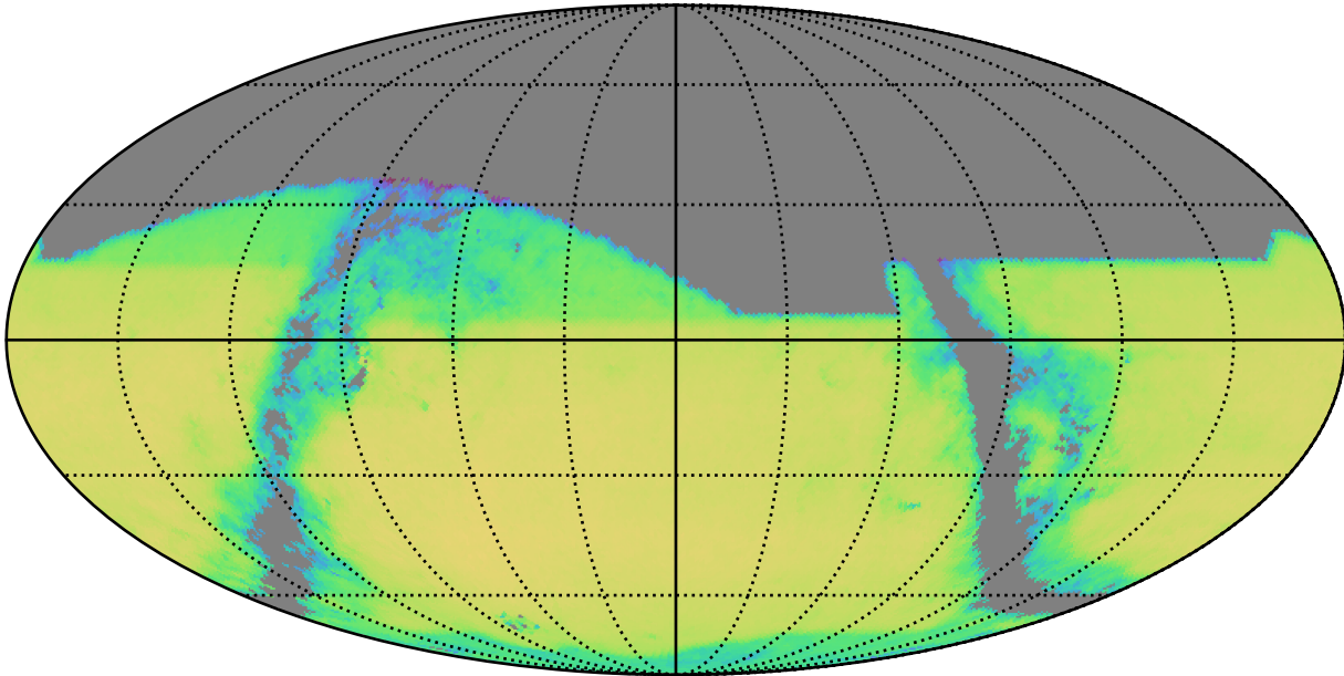
weather_cloudso16v3.4_10yrs r band and non-DD: QSONumberCountsMetric
