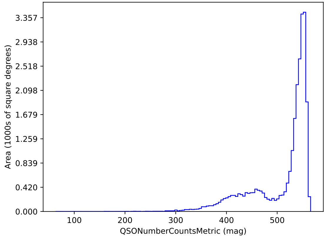
weather_cloudso16v3.4_10yrs i band and non-DD: QSONumberCountsMetric
