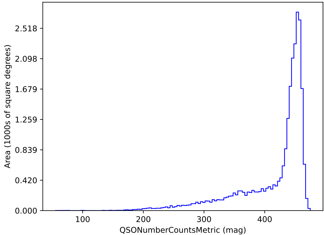
weather_cloudso16v3.4_10yrs g band and non-DD: QSONumberCountsMetric
