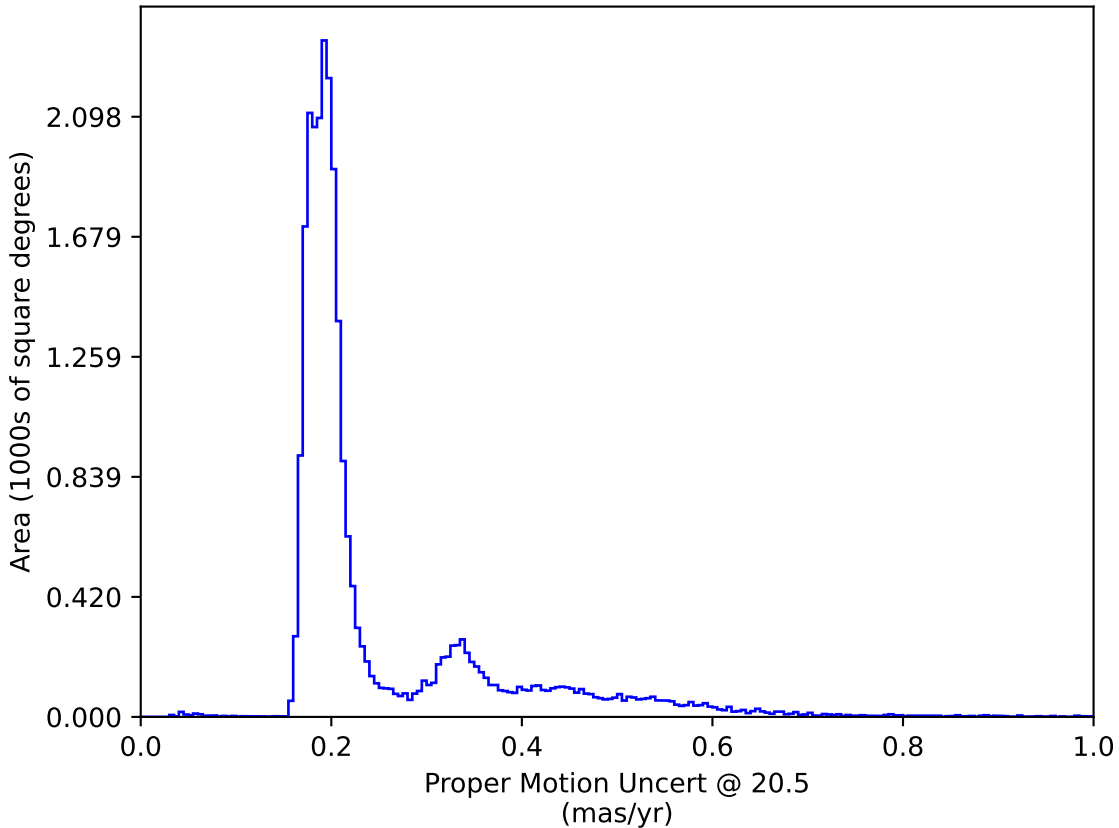
weather_cloudso16v3.4_10yrs : Proper Motion Uncert @ 20.5
