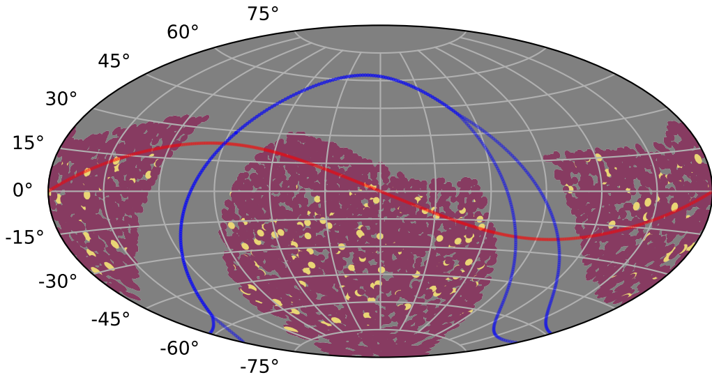
weather_cloudso16v3.4_10yrs : PrestoKNe_score_s
