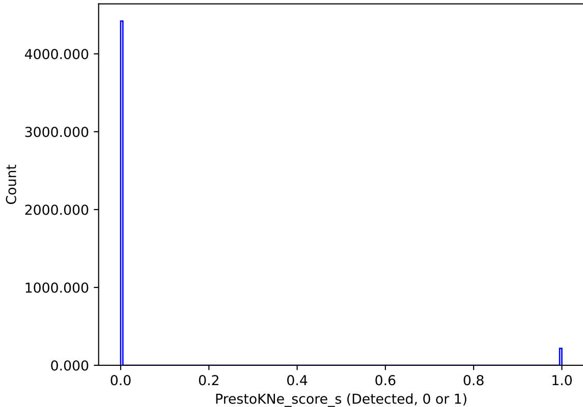
weather_cloudso16v3.4_10yrs : PrestoKNe_score_s
