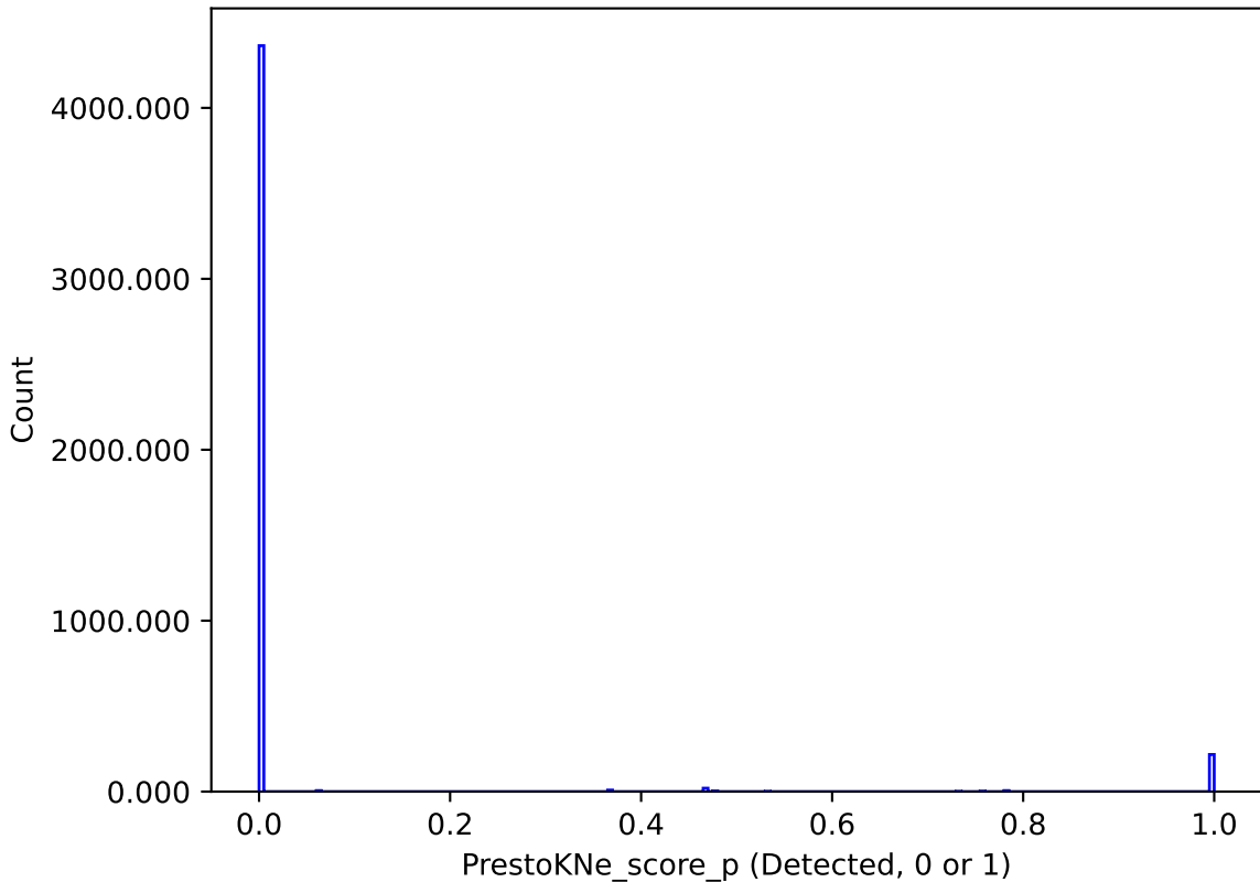
weather_cloudso16v3.4_10yrs : PrestoKNe_score_p
