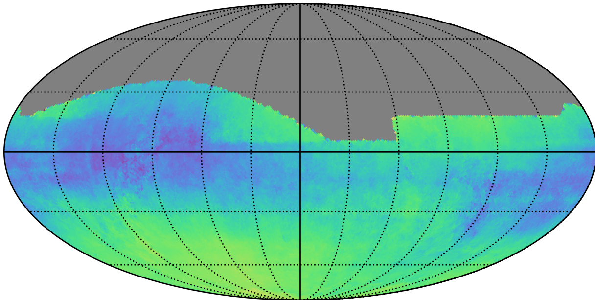
weather_cloudso16v3.4_10yrs : Parallax-DCR degeneracy @ 24.0
