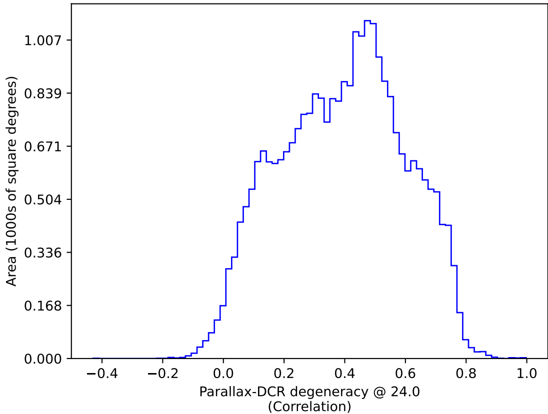
weather_cloudso16v3.4_10yrs : Parallax-DCR degeneracy @ 24.0
