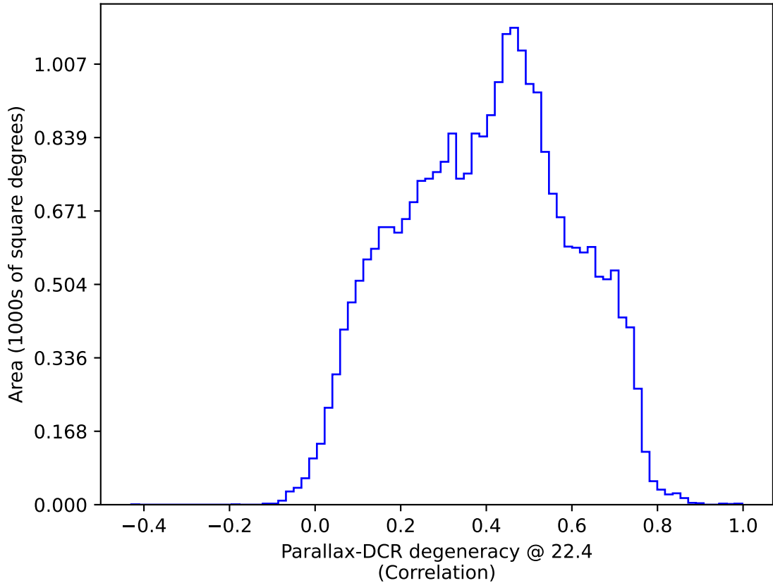
weather_cloudso16v3.4_10yrs : Parallax-DCR degeneracy @ 22.4
