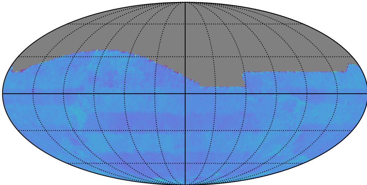
weather_cloudso16v3.4_10yrs : Normalized Proper Motion Uncert @ 24.0
