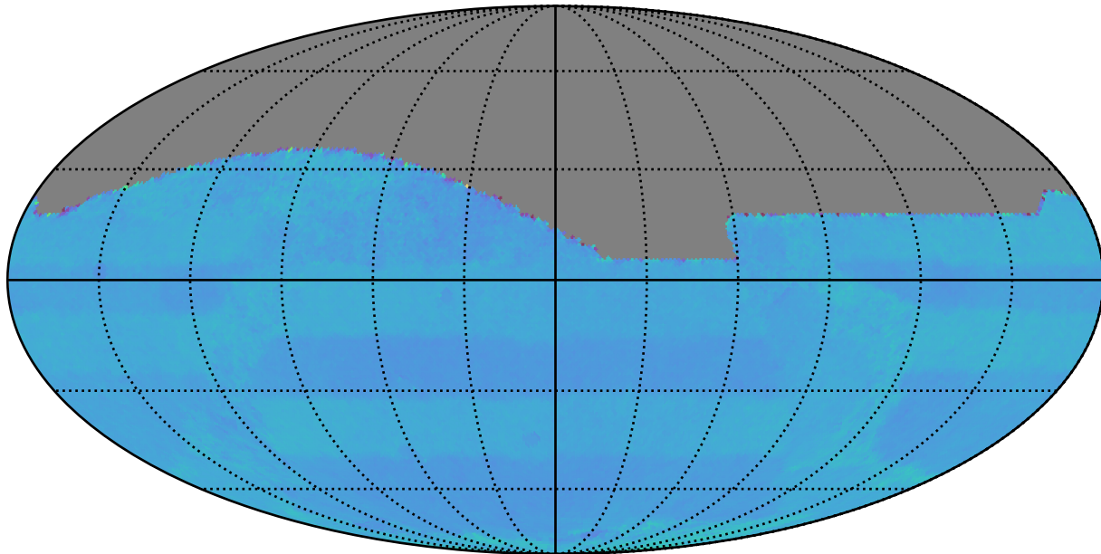
weather_cloudso16v3.4_10yrs : Normalized Proper Motion Uncert @ 20.5
