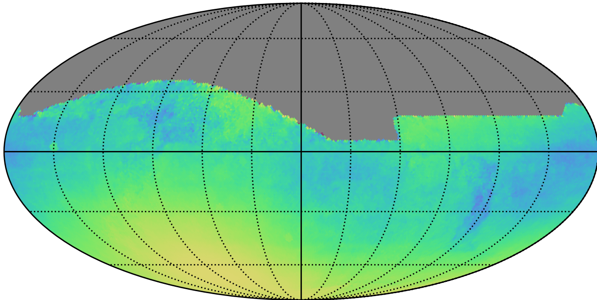
weather_cloudso16v3.4_10yrs : Normalized Parallax Uncert @ 24.0
