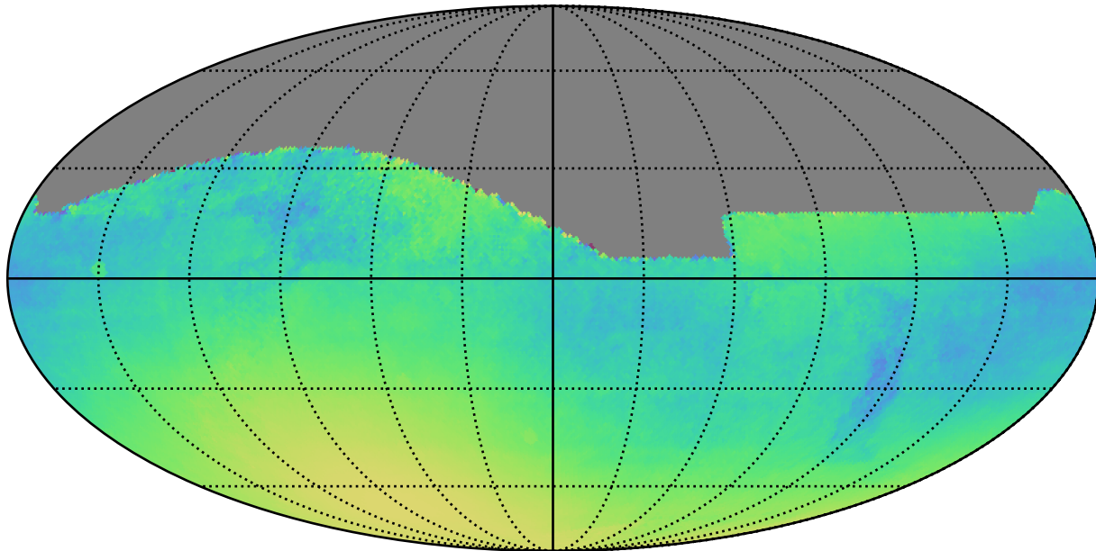
weather_cloudso16v3.4_10yrs : Normalized Parallax Uncert @ 22.4
