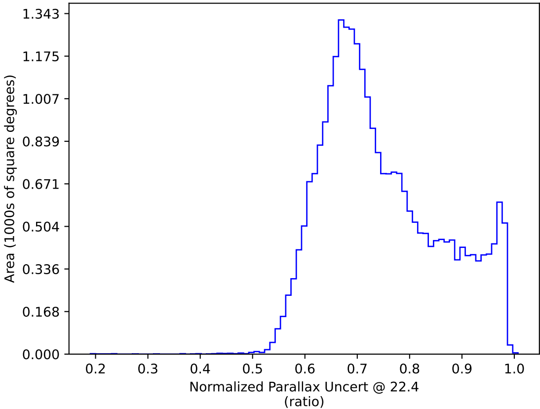
weather_cloudso16v3.4_10yrs : Normalized Parallax Uncert @ 22.4
