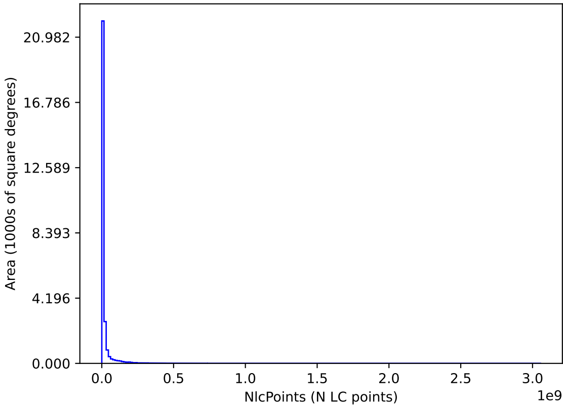
weather_cloudso16v3.4_10yrs : NlcPoints
