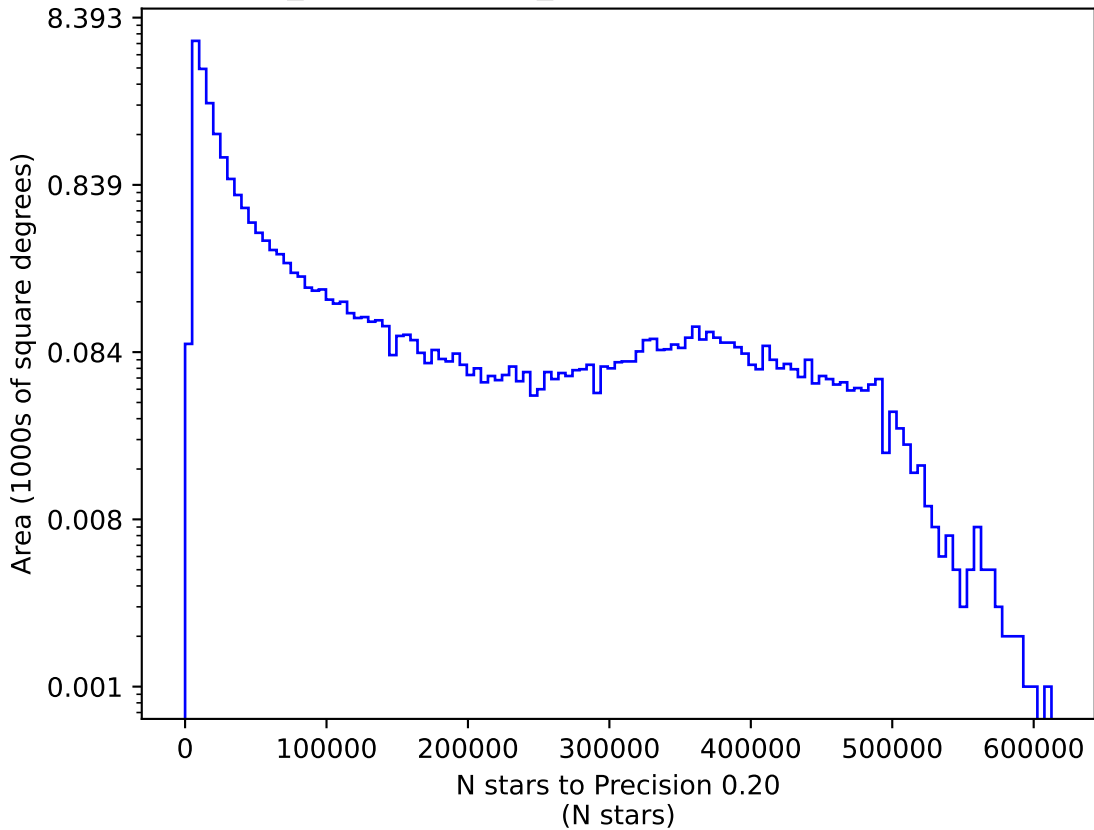
weather_cloudso16v3.4_10yrs z: N stars to Precision 0.20
