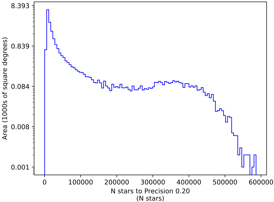
weather_cloudso16v3.4_10yrs y: N stars to Precision 0.20
