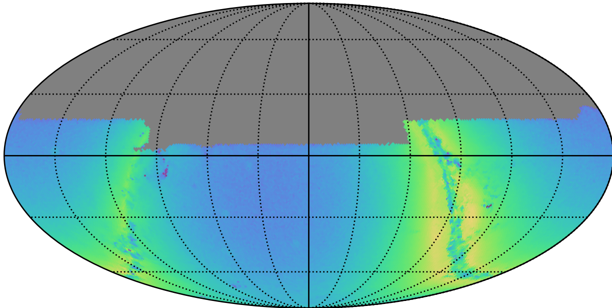
weather_cloudso16v3.4_10yrs u: N stars to Precision 0.20
