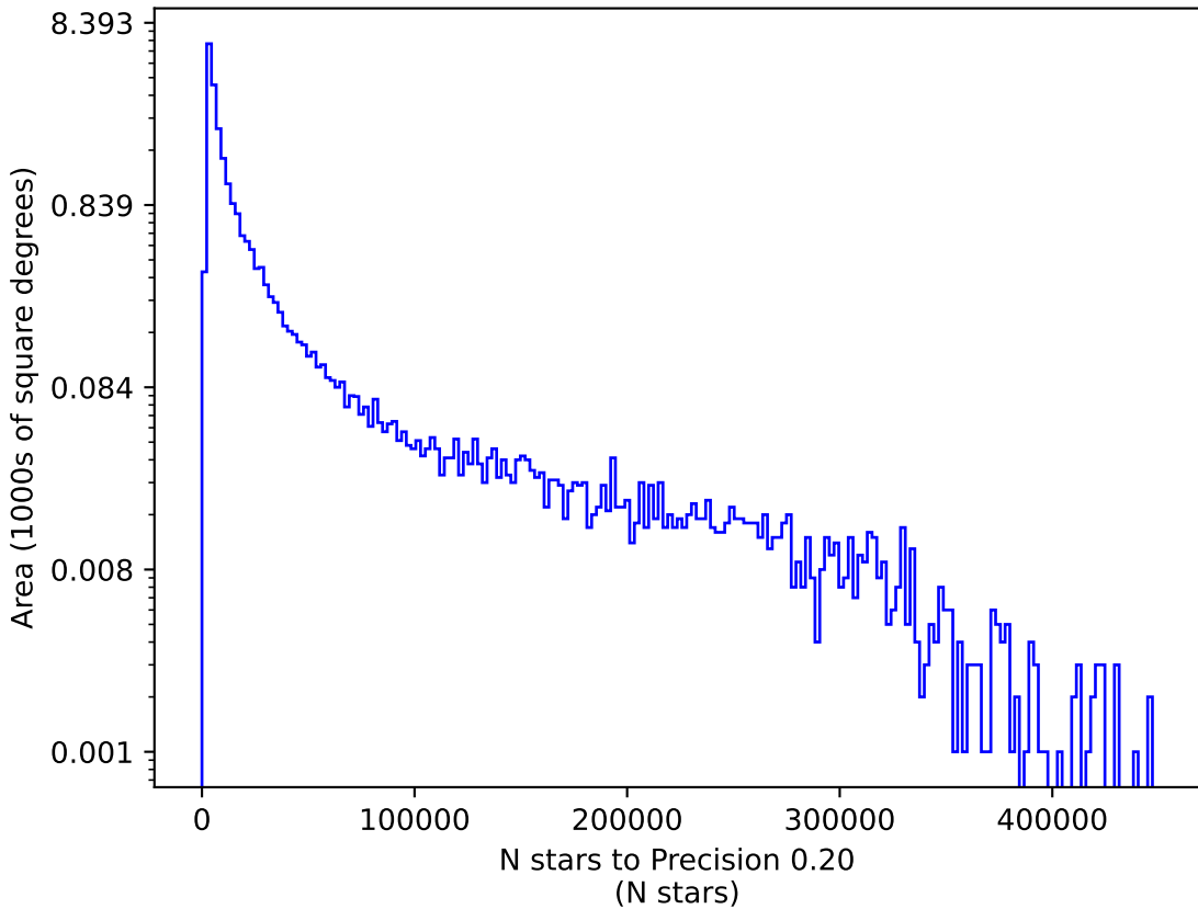
weather_cloudso16v3.4_10yrs u: N stars to Precision 0.20
