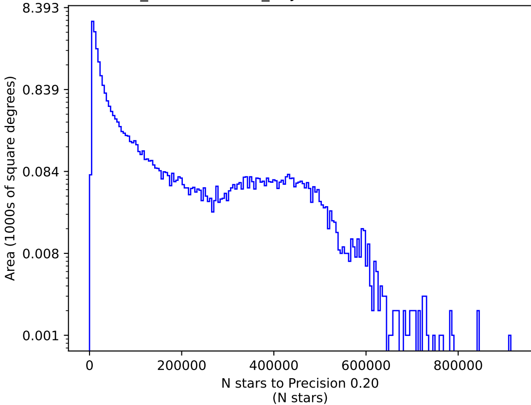
weather_cloudso16v3.4_10yrs r: N stars to Precision 0.20
