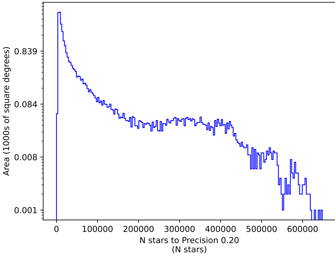
weather_cloudso16v3.4_10yrs g: N stars to Precision 0.20
