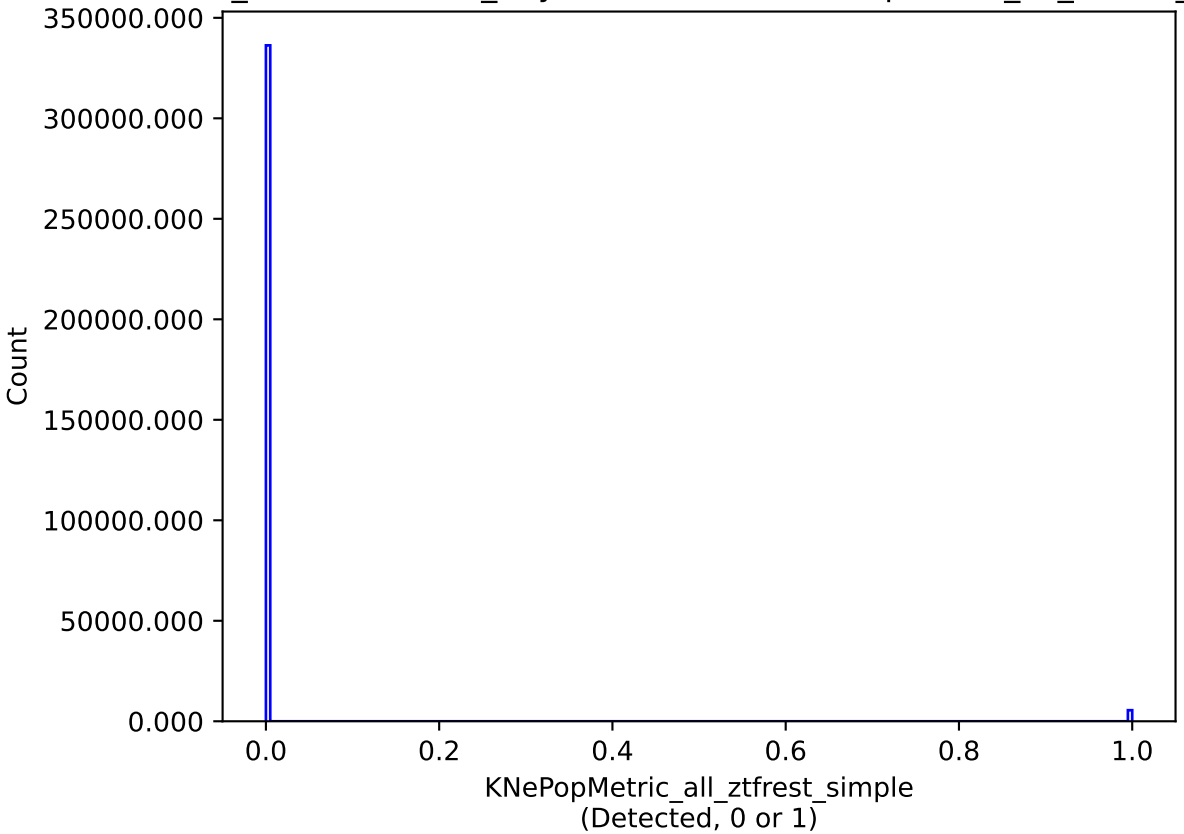
weather_cloudso16v3.4_10yrs all models: KNePopMetric_all_ztfrest_simple
