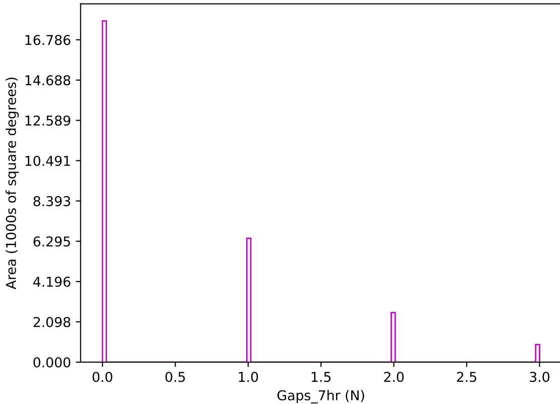
weather_cloudso16v3.4_10yrs z band: Gaps_7hr
